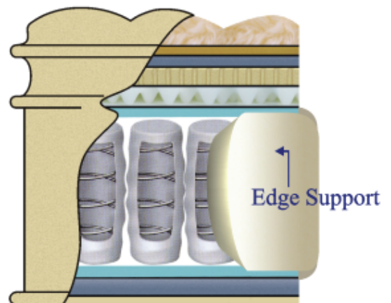
Foam-Box Construction
